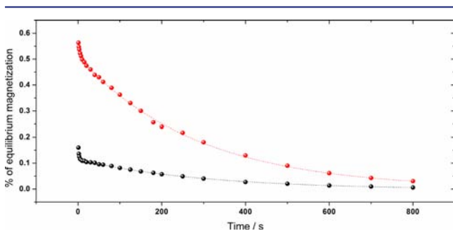
Figure 3. Observed ^{13}\text{C}_2 -DPA singlet state relaxation at 8.45 T. A T_S of 288.4 \pm 3.7 s is observed (black, the same data as in Figure 2). This is compared to a singlet state relaxation measurement where the M2S part of the MSM sequence has been applied at the ^1\text{H} resonance frequency instead of the ^{13}\text{C} resonance frequency (red), resulting in an enhancement of the acquired signal of \gamma_{\text{H}}/\gamma_{^{13}\text{C}} \approx 4 . For the singlet state relaxation using the ^1\text{H} polarization, a T_S of 282.7 \pm 3.8 s is observed. The small discrepancy in the relaxation times is likely due to subtle differences in the contributions of thermal signal in the two measurements.
