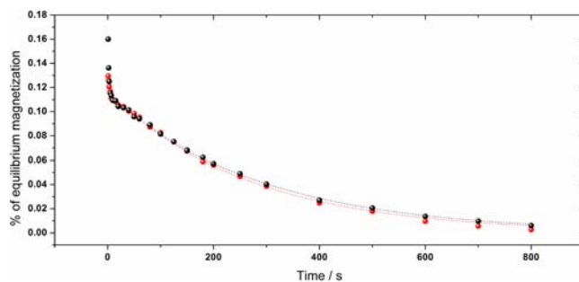
Figure 2. Observed ^{13}C_2 -DPA singlet state relaxation at 8.45 T with the MSM sequence. The singlet relaxation is preceded by a fast triplet relaxation on the order of T_1 (12 s), and after \sim 15 s a single exponential decay (singlet lifetime, T_S ) of 288.4 \pm 3.7 s is observed without ^1H decoupling (black) and a T_S of 267.1 \pm 5.4 is observed with ^1H decoupling during the delay between M2S and S2M (red). Signal is normalized against equilibrium magnetization obtained by a separate 90^\circ -acquire experiment.
